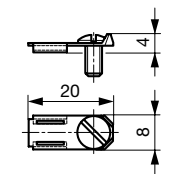
Screw-Adapter for Quick Connect-Terminals 6.3 x 0.8 mm
