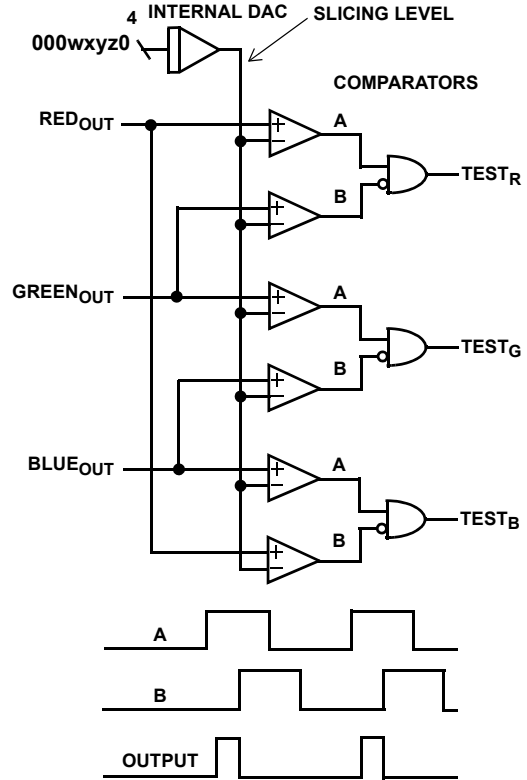
FIGURE 36. DELAY DETECTOR
