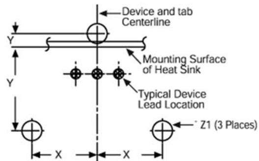
Mounting Details:
