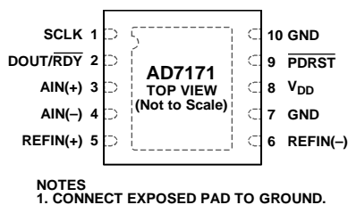
Figure 5. Pin Configuration
