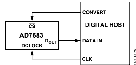
Figure 26. Connection Diagram
