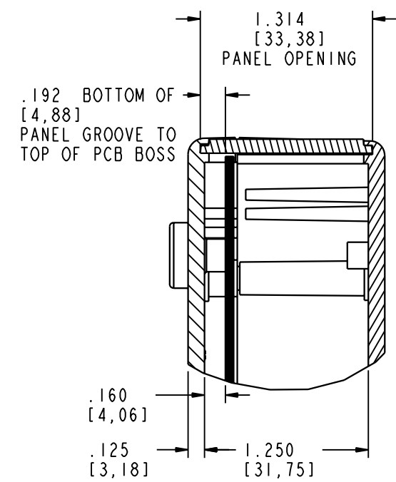
SECTION C-C SCALE 2.000
