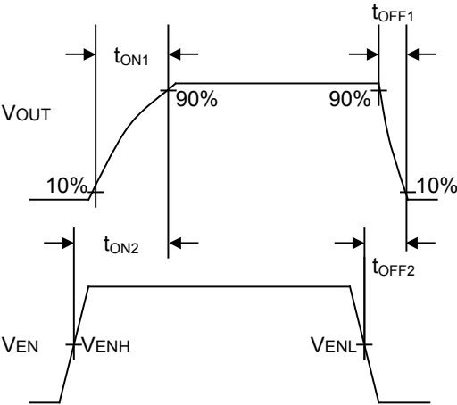
Figure 3. Timing Diagram(BD2066FJ)
