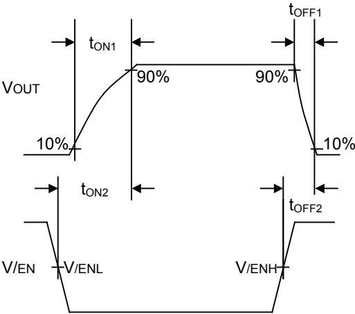
Figure 2. Timing Diagram(BD2062FJ)
