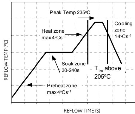
Figure 19. Reflow Profile for Tin/Lead (Sn/Pb) process.
