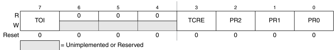
Figure 14-16. Timer System Control Register 2 (TSCR2)
