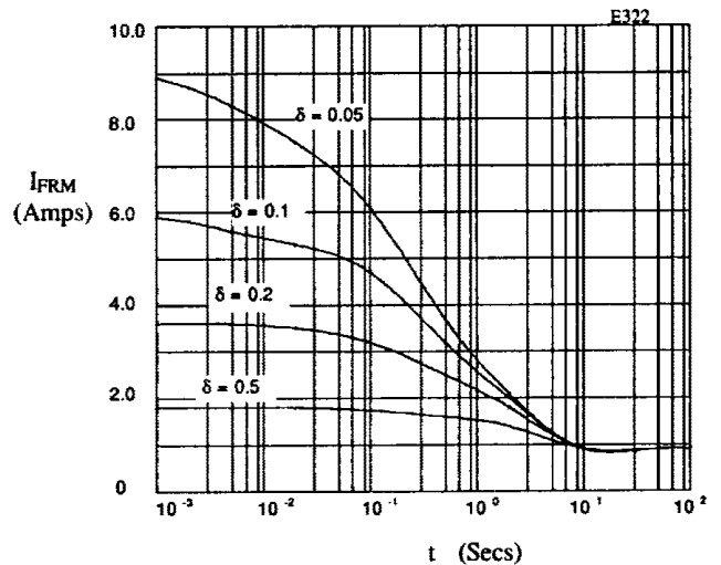
Fig 8. Typical repetitive forward current as a function of pulse width at 100^\circ\text{C} ; R_{\theta JL} = 95^\circ\text{C/W} ; V_{RWM} during 1 - \delta .
