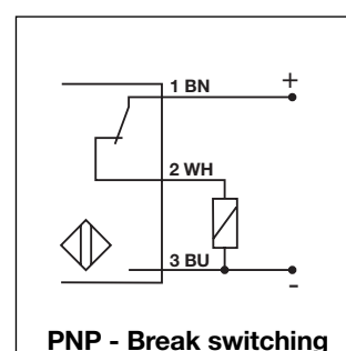
PNP - Break switching
