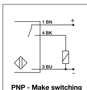
PNP - Make switching
