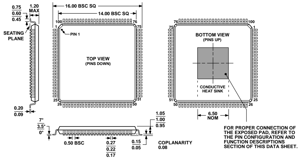
Figure 87. 100-Lead Thin Quad Flat Package, Exposed Pad [TQFP_EP] (SV-100-1) Dimensions shown in millimeters
