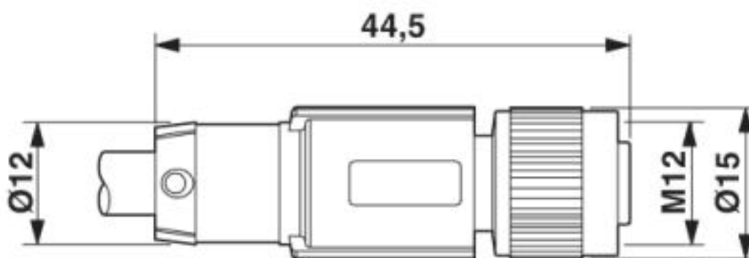
Dimensional drawing
