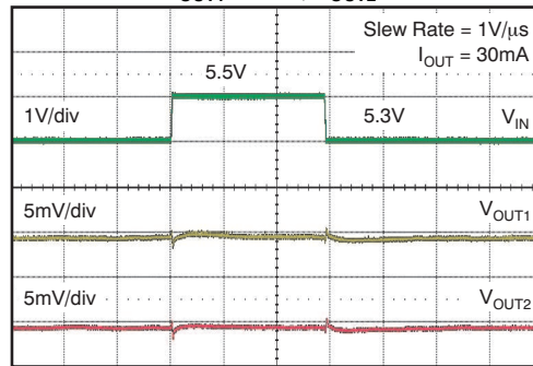
Time (200 \mu\text{s} /div) Figure 60.
