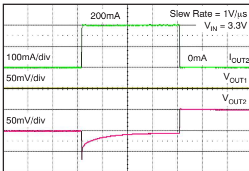
Time (50 \mu\text{s} /div) Figure 63.
