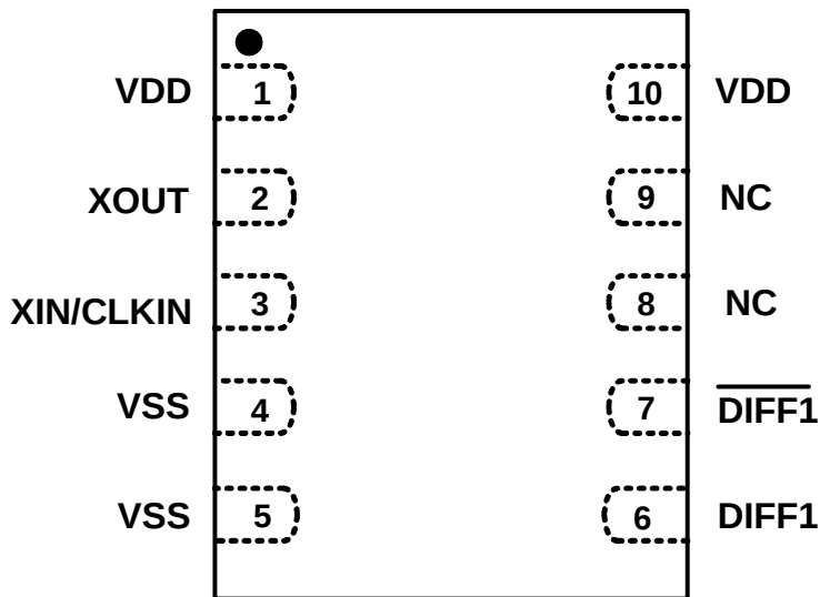
Figure 6. 10-Pin TDFN
