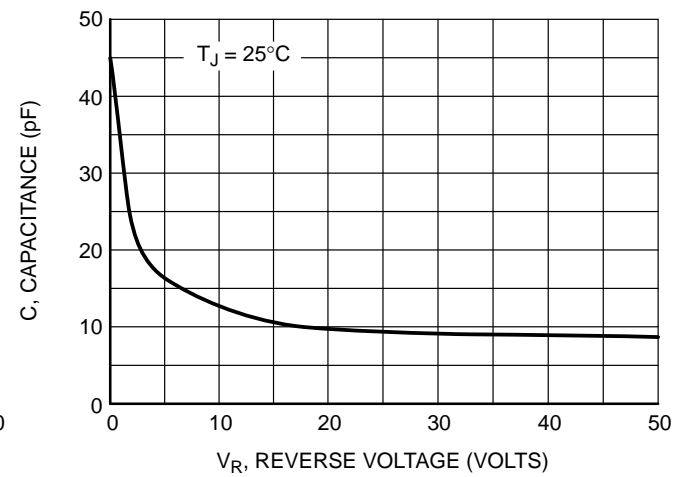
Figure 8. Typical Capacitance
