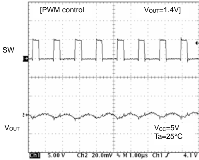
Figure 67. SW Waveform ( I_o=500\text{mA} )
