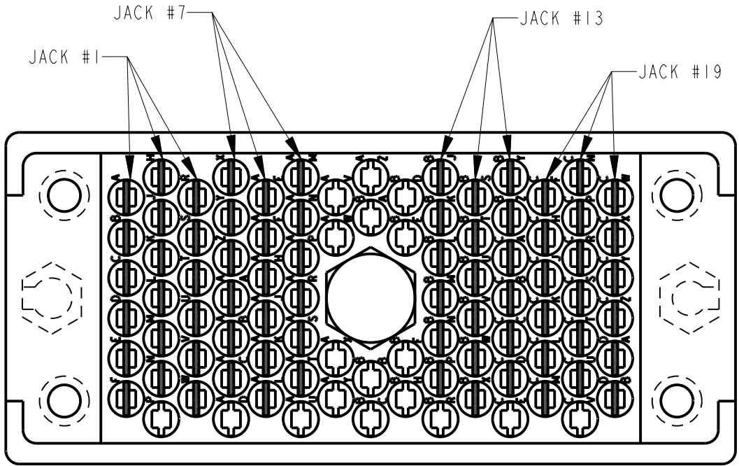
STANDARD AUDIO CONFIGURATION WIRING (S.A.C.) WIRING VIEW - ROTATED 180° (NORMALS AT JACKS)
