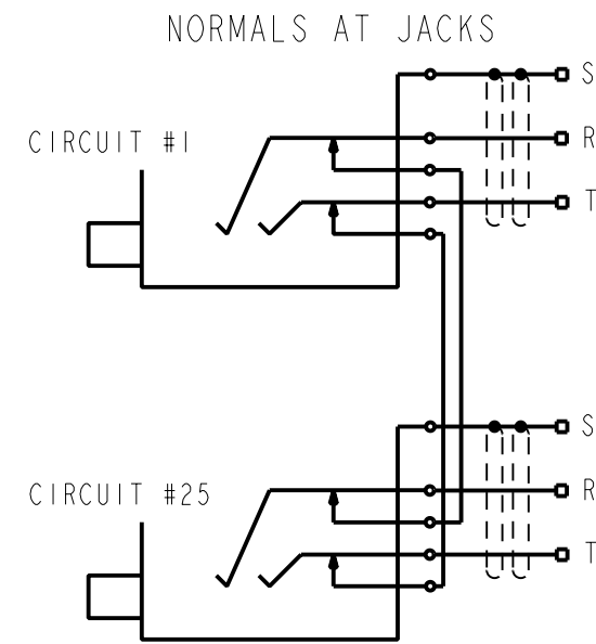
STANDARD AUDIO CONFIGURATION WIRING (S.A.C.) WIRING VIEW - ROTATED 180° (NORMALS AT JACKS)
