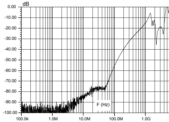
Figure 9. Analog crosstalk
