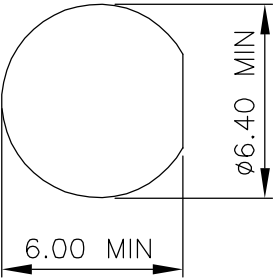
RECOMMENDED MOUNTING HOLE DIM'S
