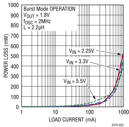
1A Buck Power Loss vs I_{LOAD} , V_{OUT} = 1.8V
