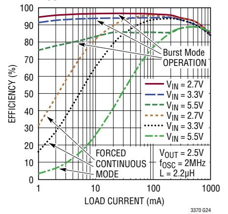
1A Buck Efficiency vs I_{LOAD} , V_{OUT} = 2.5V
