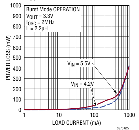
1A Buck Power Loss vs I_{LOAD} , V_{OUT} = 3.3V
