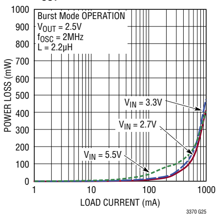
1A Buck Power Loss vs I_{LOAD} , V_{OUT} = 2.5V
