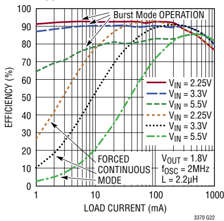
1A Buck Efficiency vs I_{LOAD} , V_{OUT} = 1.8V
