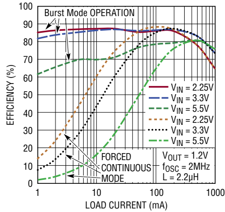
1A Buck Efficiency vs I_{LOAD} , V_{OUT} = 1.2V
