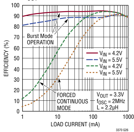
1A Buck Efficiency vs I_{LOAD} , V_{OUT} = 3.3V
