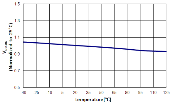
Figure 7. V DD-ON vs. Temperature
