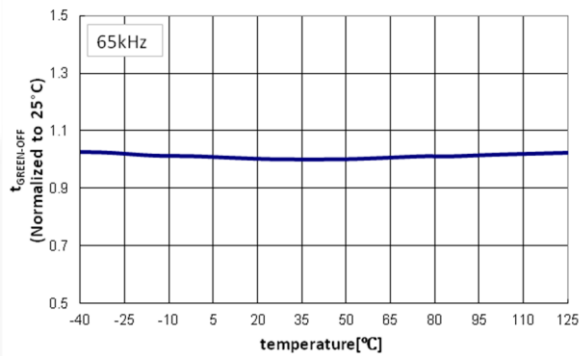
Figure 9. t GREEN-OFF vs. Temperature
