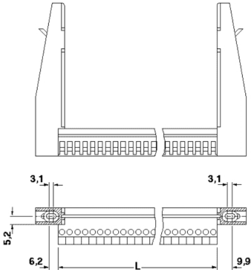
Dimensional drawing
