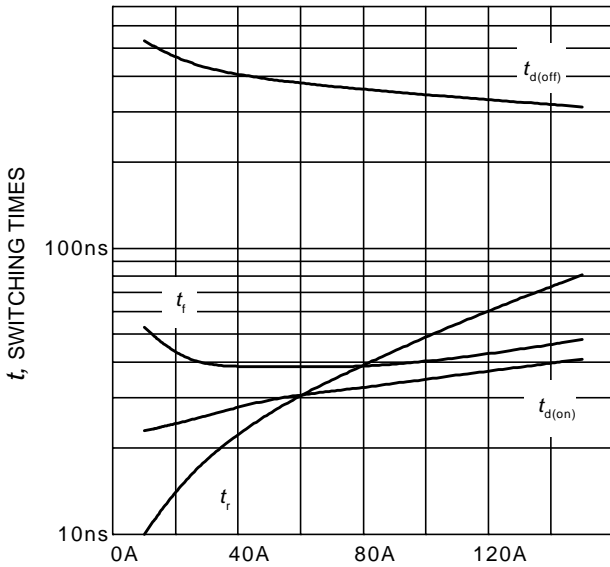
Figure 9. Typical switching times as a function of collector current (inductive load, T_J=175^\circ\text{C} , V_{CE} = 400\text{V} , V_{GE} = 0/15\text{V} , r_G = 5\Omega , Dynamic test circuit in Figure E)
