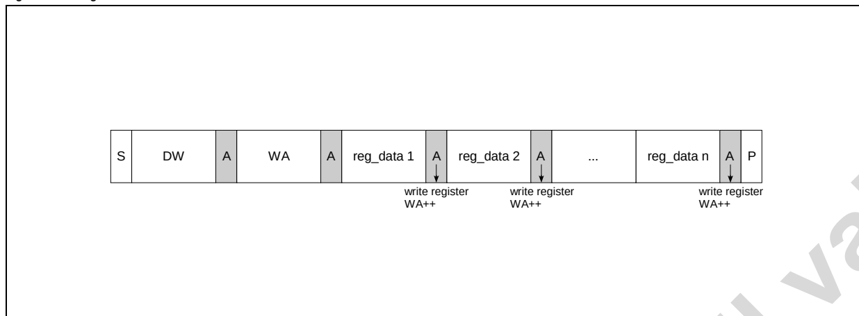
Figure 16. Page Write
