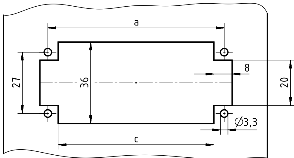
panel cut out for Han Snap Adapter
