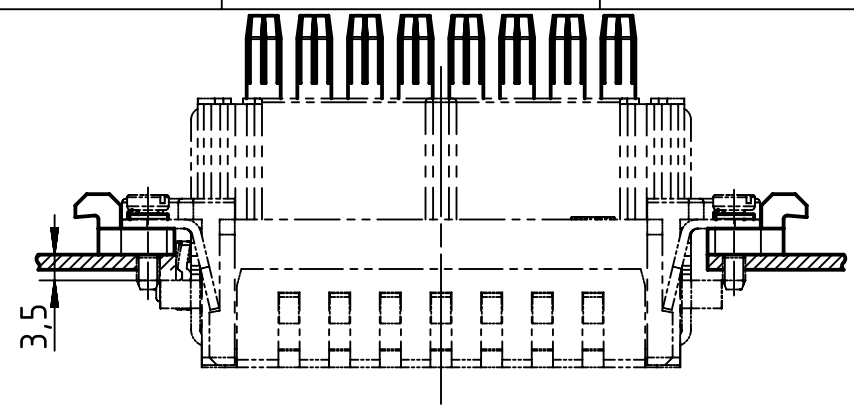
panel cut out for Han Snap Adapter
