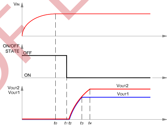
Figure 5. Startup scenario #2.
