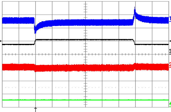
Figure 23. Output voltage response to lout1 load current step-change of 3.75 A (50%-75%-50%) at lout2 = 5 A and Vin = 48 V. Ch1 = Vout1 (50 mV/div), Ch2 = Vout2 (50 mV/div), Ch3 = lout1 (10 A/div), Ch4 = lout2 (10 A/div). Current slew rate: 0.1 A/ \mu s, Co = 10 \mu F tantalum + 1 \mu F ceramic. Time scale: 0.5 ms/div.
