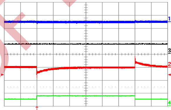
Figure 26. Output voltage response to lout2 load current step-change of 2.5 A (50%-75%-50%) at lout1 = 7.5 A and Vin = 48 V. Ch1 = Vout1 (100 mV/div), Ch2 = Vout2 (100 mV/div), Ch3 = lout1 (10 A/div), Ch4 = lout2 (10 A/div). Current slew rate: 5 A/ \mu s, Co = 300 \mu F tantalum + 1 \mu F ceramic. Time scale: 0.5 ms/div.
