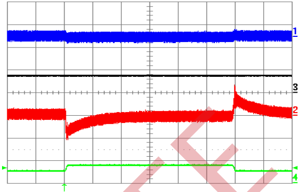
Figure 24. Output voltage response to lout2 load current step-change of 2.5 A (50%-75%-50%) at lout1 = 7.5 A and Vin = 48 V. Ch1 = Vout1 (50 mV/div), Ch2 = Vout2 (50 mV/div), Ch3 = lout1 (10 A/div), Ch4 = lout2 (10 A/div). Current slew rate: 0.1 A/ \mu s, Co = 10 \mu F tantalum + 1 \mu F ceramic. Time scale: 0.5 ms/div.
