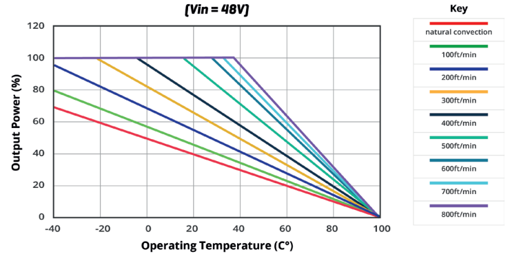
TEMPERATURE DERATING CURVE VHB350-D48-S12 without heatsink ( V_{in} = 48V )
