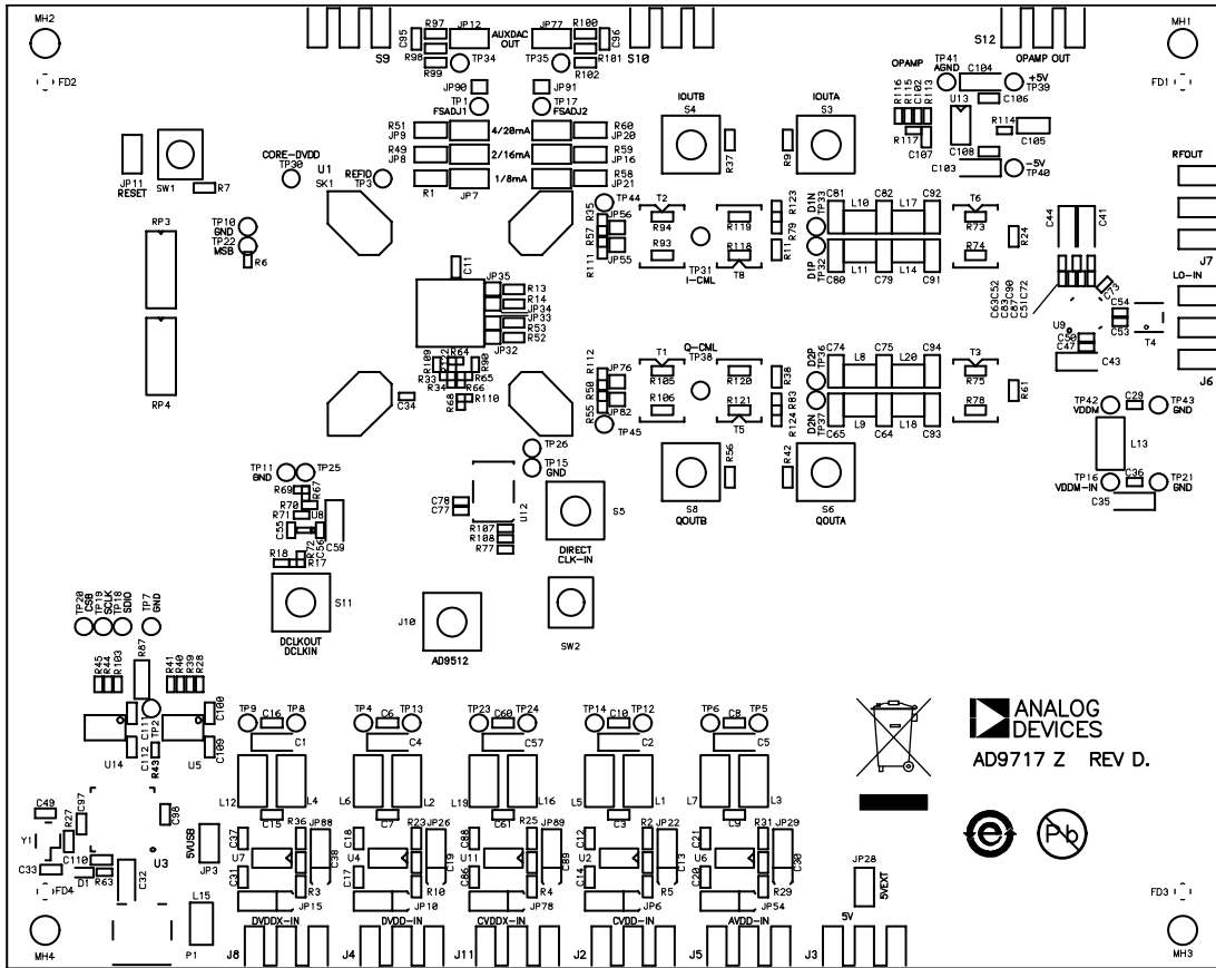
Figure 129. Silkscreen—Primary Side
