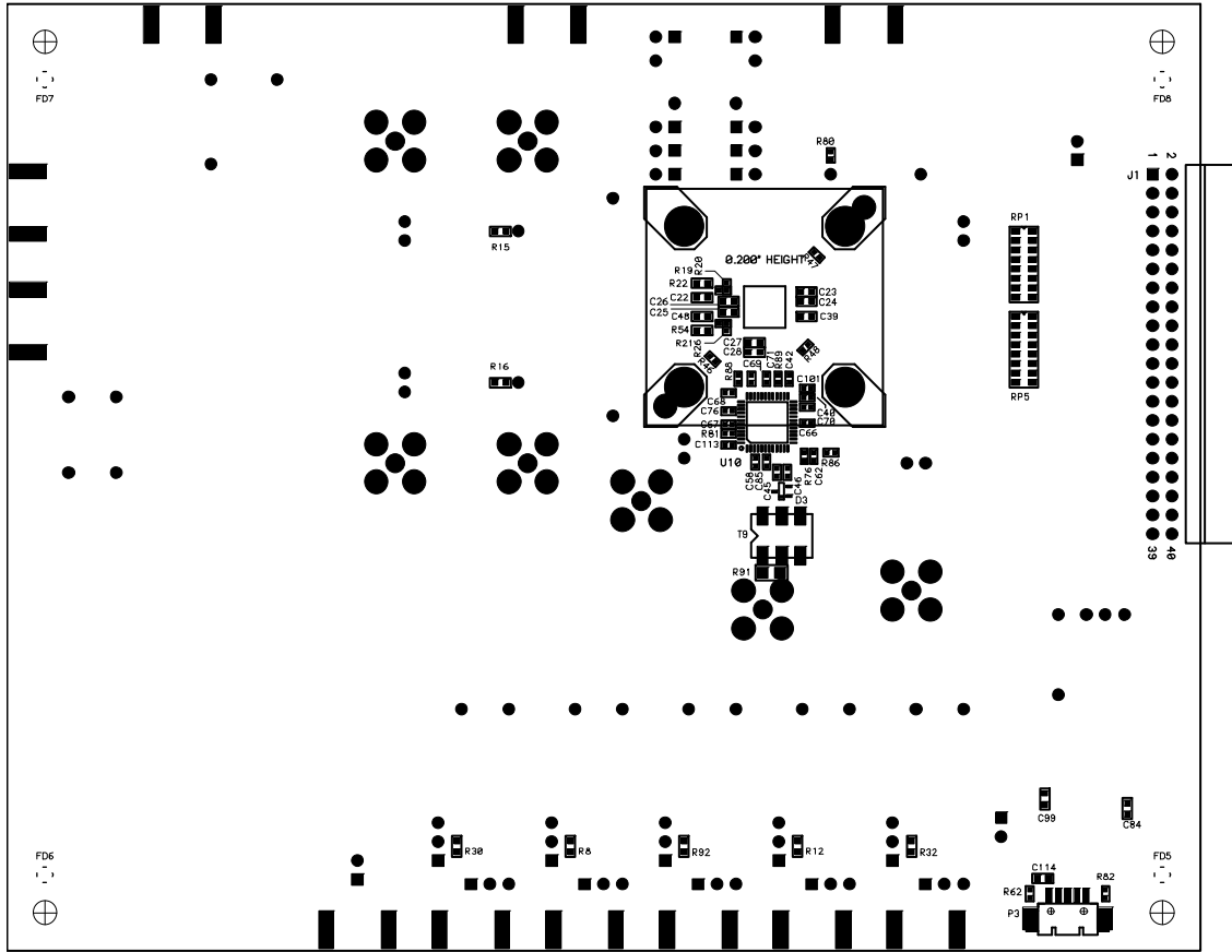
Figure 123. Assembly—Secondary Side
