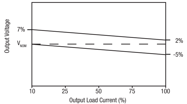
12V Output
