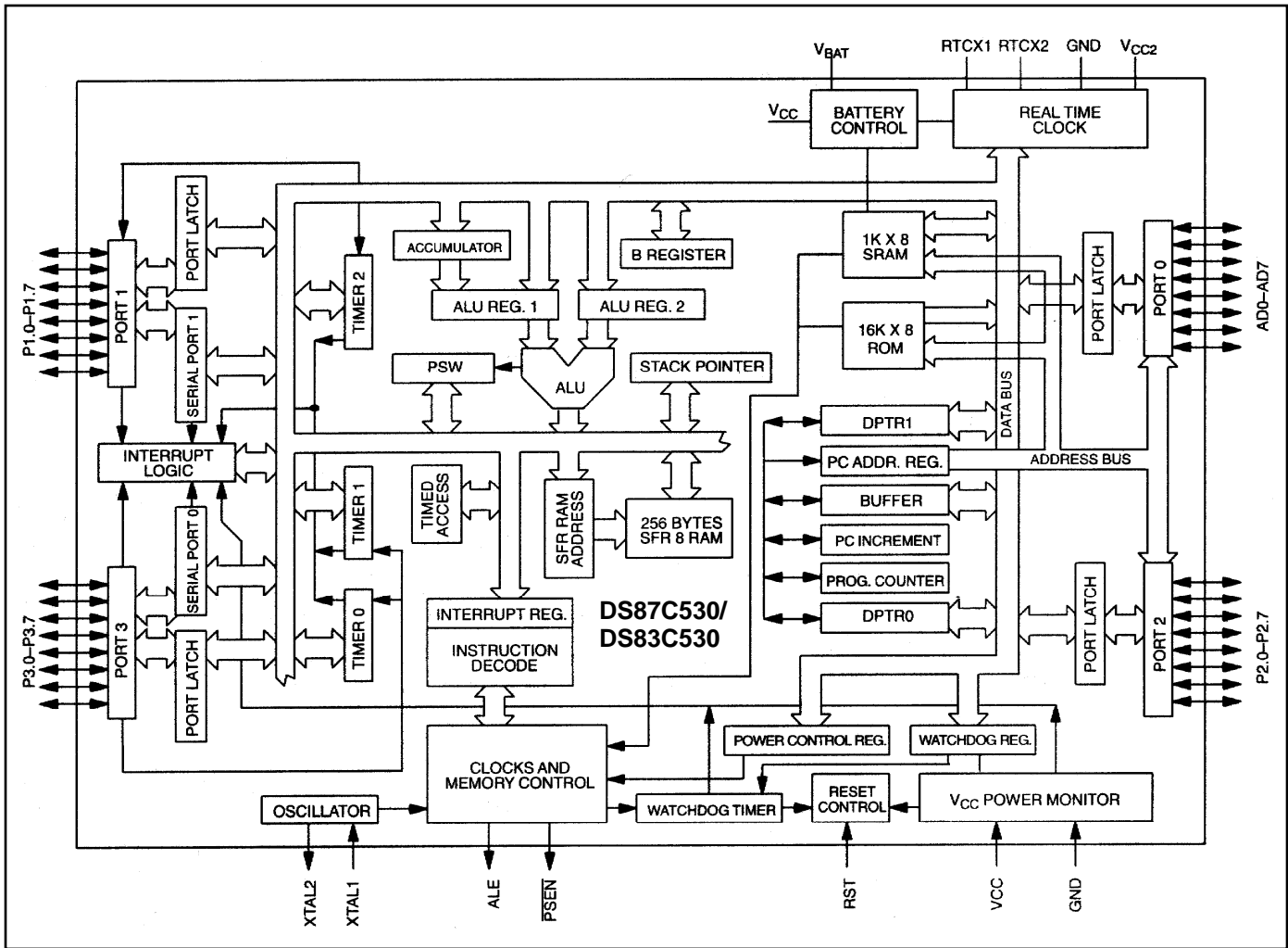
Figure 1. Block Diagram
