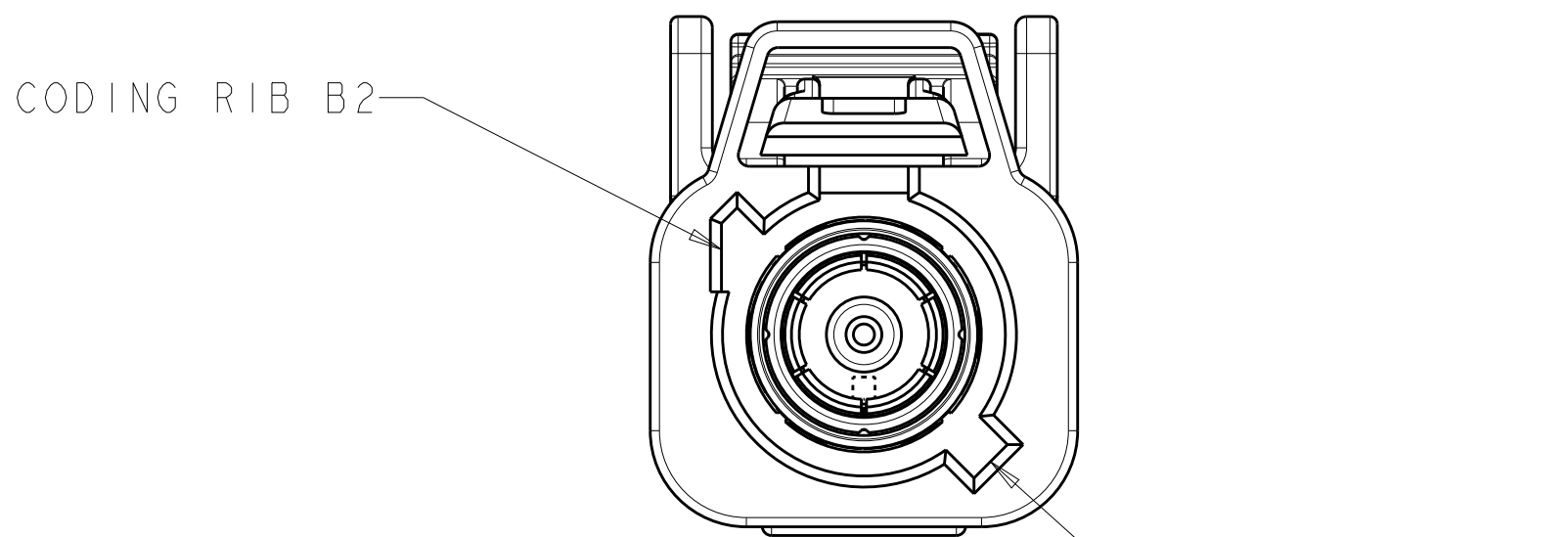
DETAIL I
