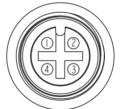
Conn. 2 Pin Assignments Front View
