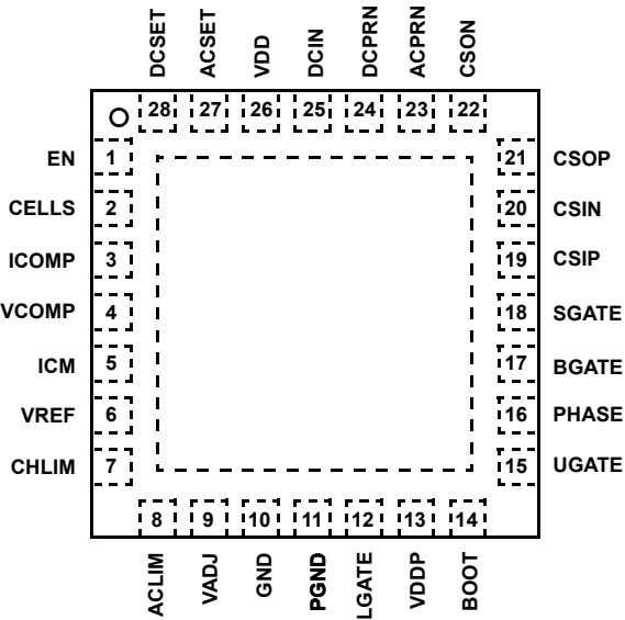
ISL6255, ISL6255A (28 LD QFN) TOP VIEW
