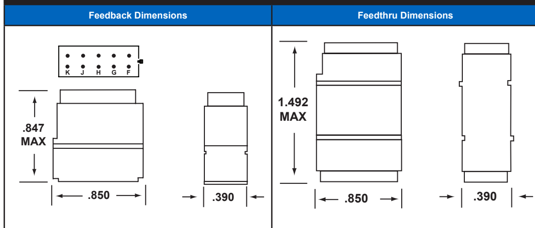
Terminal Junction Module Dimensions
