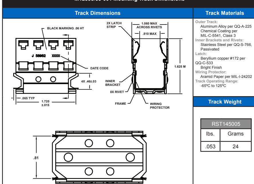
M12883/53-001 Mounting Track Dimensions
