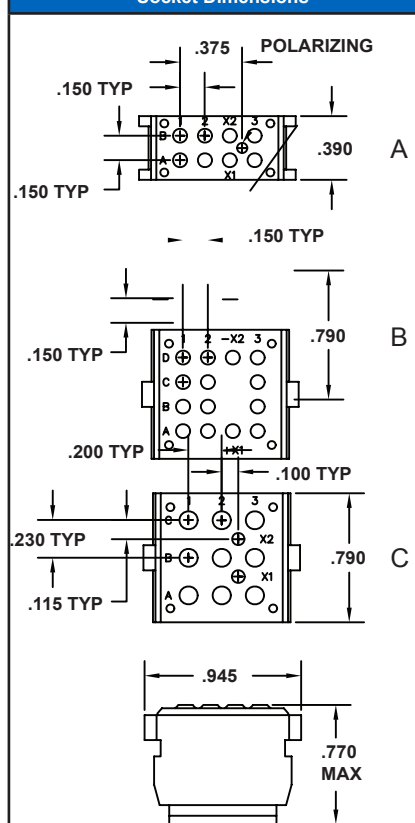
Socket Dimensions
