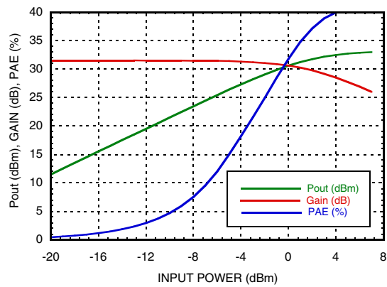
Power Compression @ 3.5 GHz
