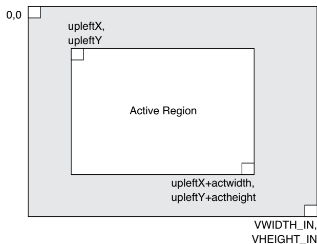
Figure 2-2. 2D Edge Detector IP Core Active Regions
