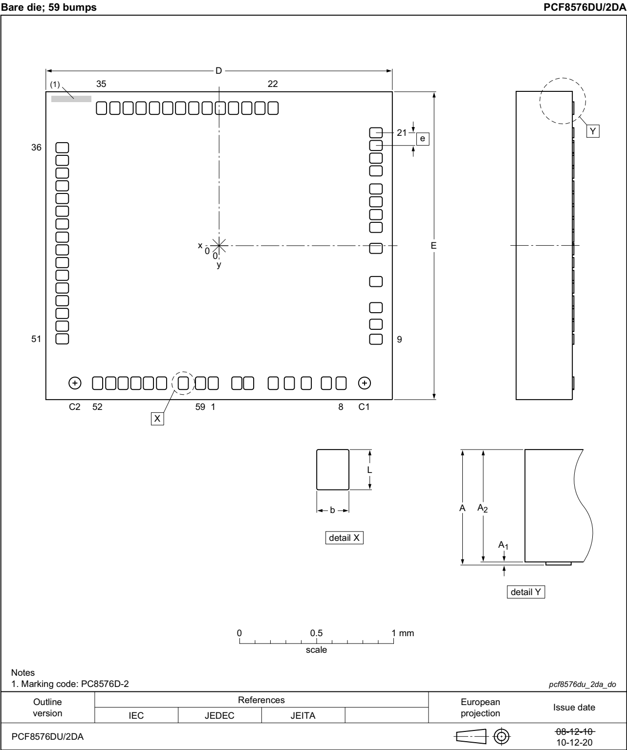
Fig 27. Bare die outline PCF8576DU/2DA (for dimensions see Table 24)
