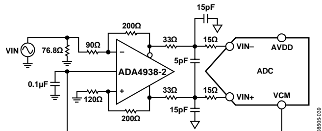
Figure 66. Differential Input Configuration Using the ADA4938-2
