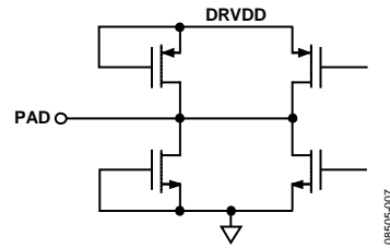
Figure 57. Digital Output
