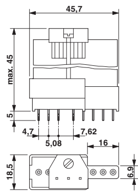
Dimensional drawing
