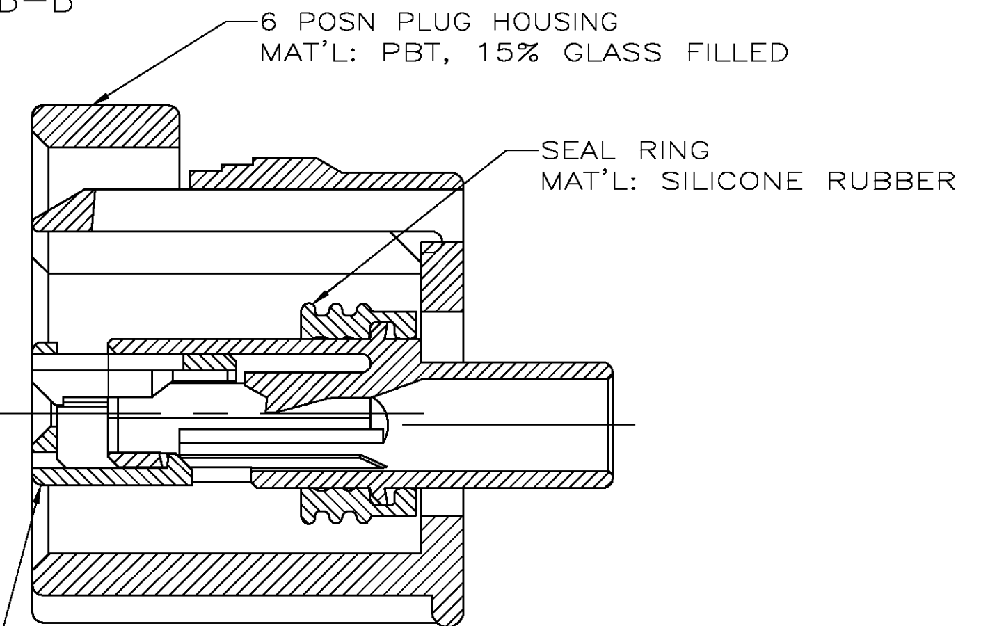
VIEW B-B
