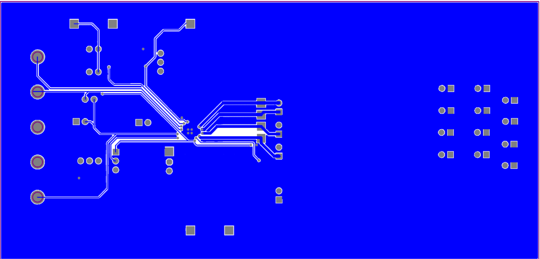
FIGURE 3. BOTTOM LAYER
