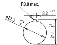
Mounting Hole
