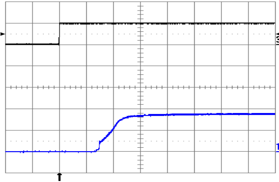
Fig. 1.8V.9: Turn-on transient at full rated load current (resistive) with no output capacitor at V_{in} = 24V , triggered via ON/OFF pin. Top trace: ON/OFF signal (5 V/div.). Bottom trace: output voltage (1 V/div.). Time scale: 1 ms/div.
