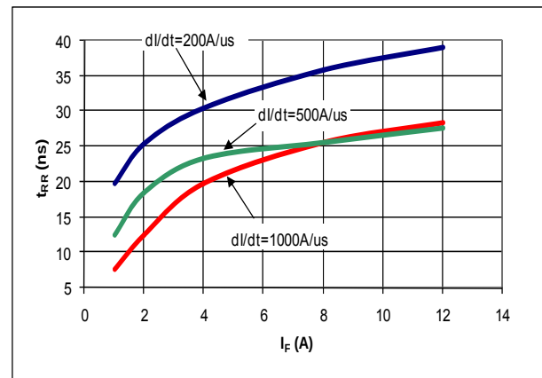
Figure 6. Typical t_{RR} vs I_F at T_J = 125^\circ
