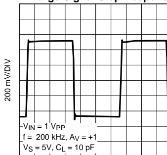
800 ns/DIV Figure 35.
