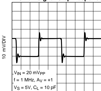
200 ns/DIV Figure 34.
