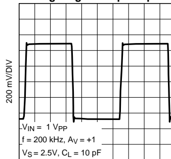
800 ns/DIV Figure 33.
