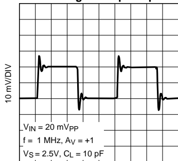
200 ns/DIV Figure 32.
