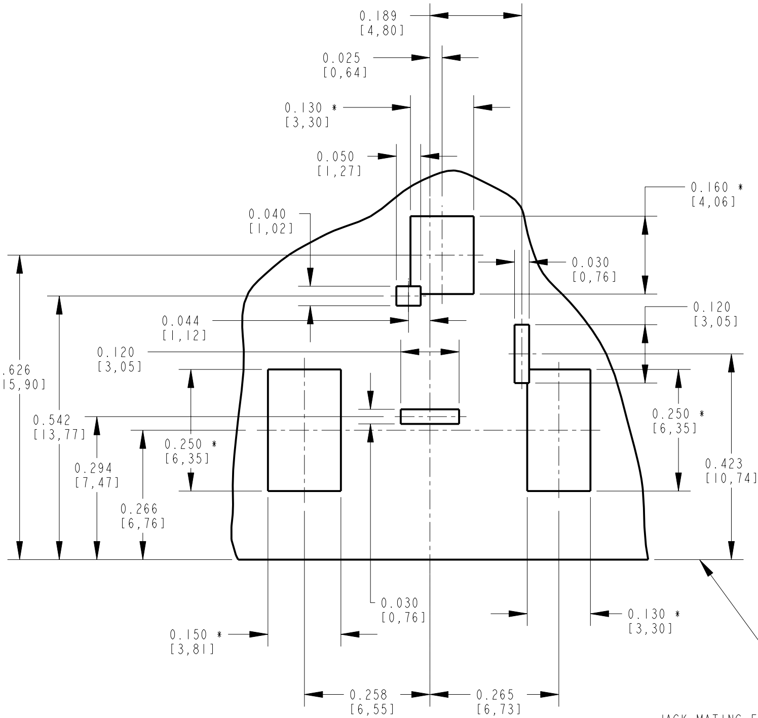
RECOMMENDED PC BOARD LAYOUT (COMPONENT SIDE)
