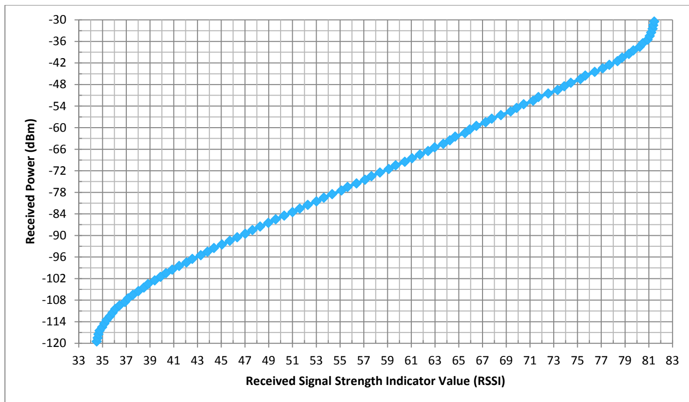
Figure 5.5: Typical input power vs. RSSI value
