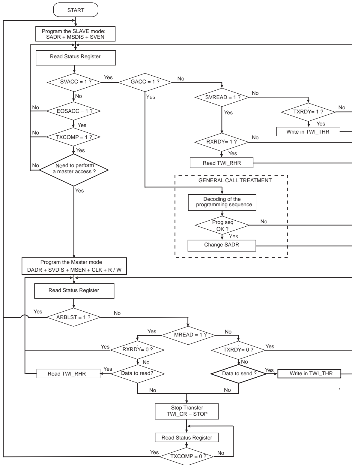
Figure 35-22. Multi-master Flowchart
