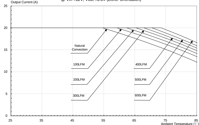
Figure 44: Output current vs. ambient temperature and air velocity @ Vin=12V, Vout=3.3V(Either Orientation)
