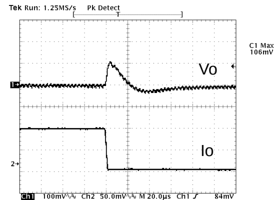
Figure 22: Typical transient response to step load change at 5A/\mu S from 100% to 50% of I_o , max at 12Vin, 2.5V out ( C_{out} = 1\mu F + 100\mu F ceramic, 470uF poscap).
