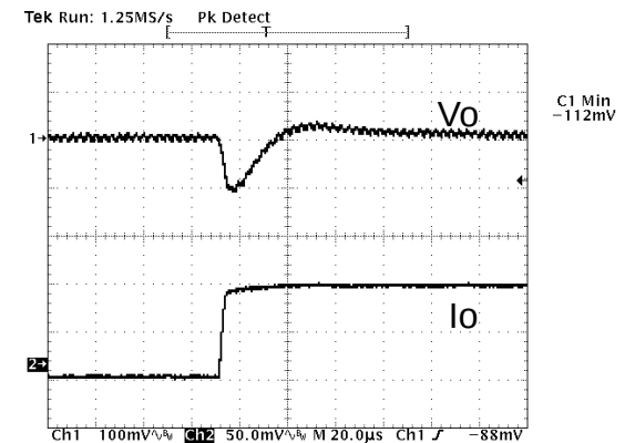
Figure 23: Typical transient response to step load change at 5A/\mu S from 50% to 100% of I_o , max at 12Vin, 2.5V out ( C_{out} = 1\mu F + 100\mu F ceramic, 470uF poscap).
