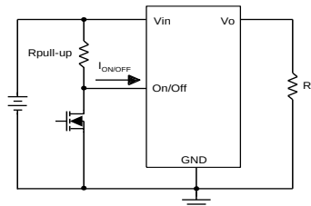
Figure 32: Negative remote On/Off implementation
