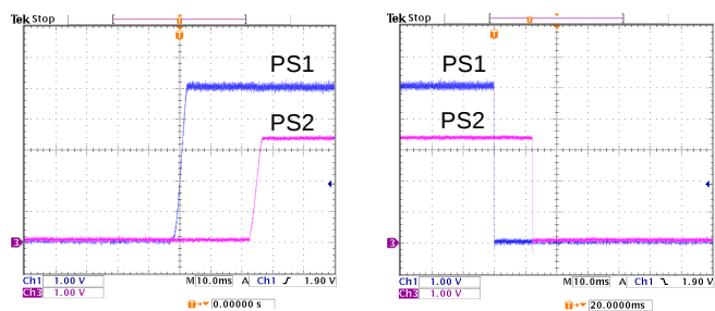
Figure 37: Sequential start-up
