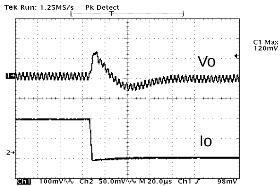
Figure 24: Typical transient response to step load change at 5A/\mu s from 100% to 50% of I_o , max at 12Vin, 5.0V out ( C_{out} = 1\mu F + 100\mu F ceramic, 470μF poscap).
