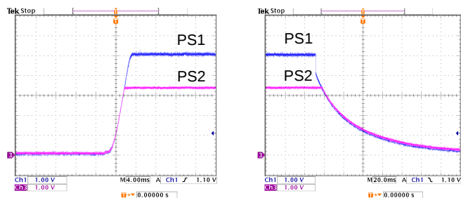
Figure 37: Sequential start-up
