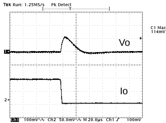
Figure 20: Typical transient response to step load change at 5A/\mu S from 100% to 50% of I_o , max at 12Vin, 1.2V out ( C_{out} = 1\mu F + 100\mu F ceramic, 470uF poscap).
