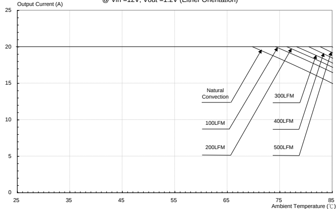
Figure42: Output current vs. ambient temperature and air velocity @ Vin=12V, Vout=1.2V(Either Orientation)
