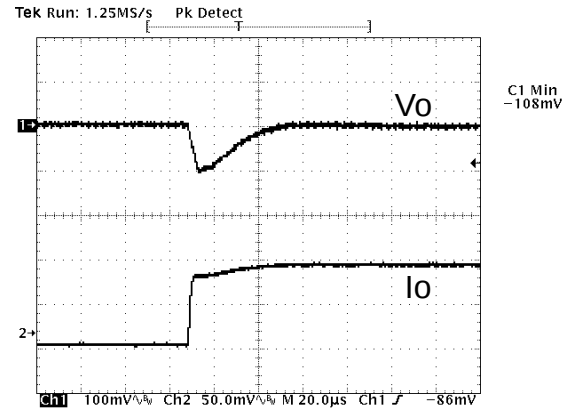
Figure 19: Typical transient response to step load change at 5A/\mu S from 50% to 100% of I_o , max at 12Vin, 0.75V out ( C_{out} = 1\mu F + 100\mu F ceramic, 470uF poscap).
