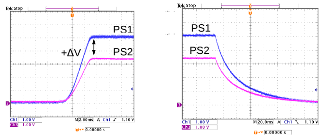
Figure 39: Ratio-metric
