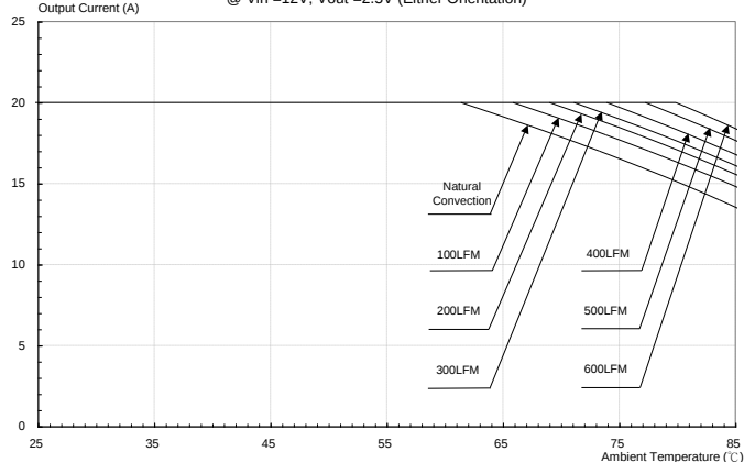
Figure 43: Output current vs. ambient temperature and air velocity @ Vin=12V, Vout=2.5V(Either Orientation)
