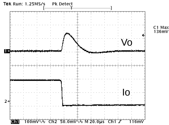
Figure 18: Typical transient response to step load change at 5A/\mu S from 100% to 50% of I_o , max at 12Vin, 0.75V out ( C_{out} = 1\mu F + 100\mu F ceramic, 470uF poscap).
