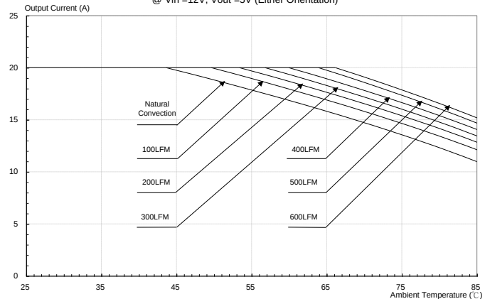
Figure 45: Output current vs. ambient temperature and air velocity @ Vin=12V, Vout=5.0V(Either Orientation)
